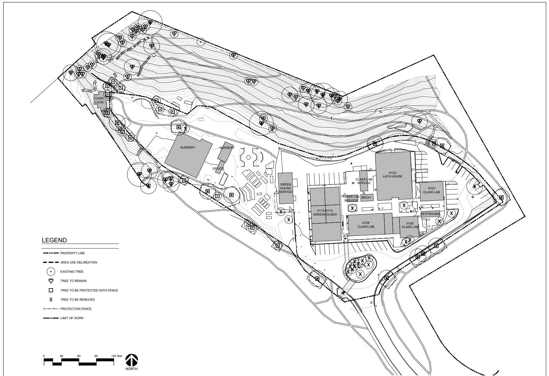
Figure 2 Current Landscape Horticulture Complex Site Plan
