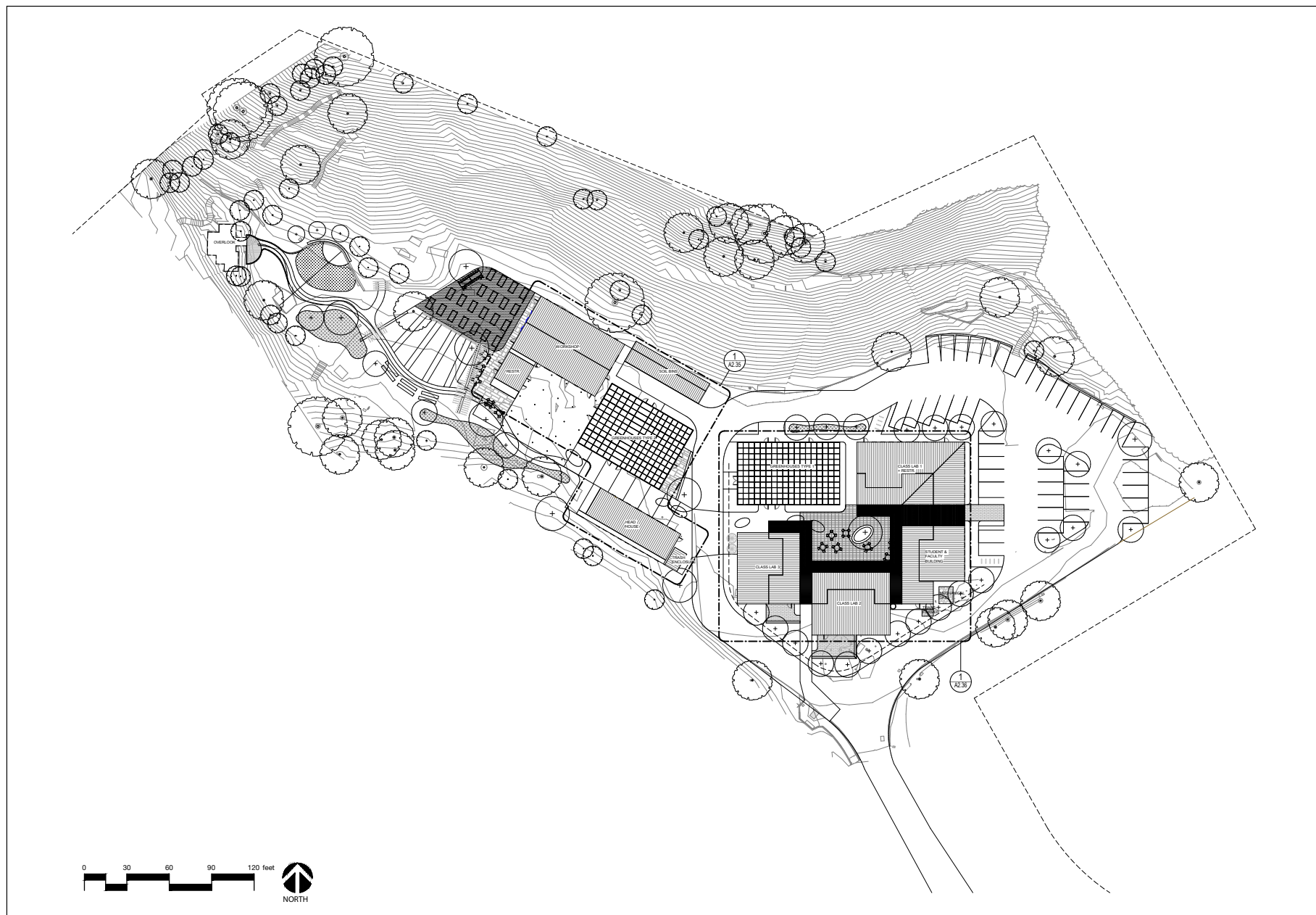
Figure 3 Proposed Landscape Horticulture Complex Site Plan
